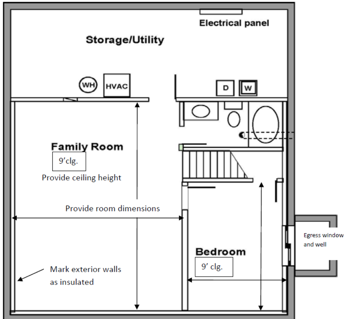
Sample Plan
