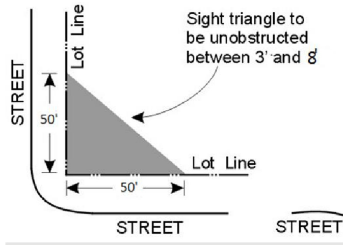
Figure 5-2017.1 Site Triangle.
