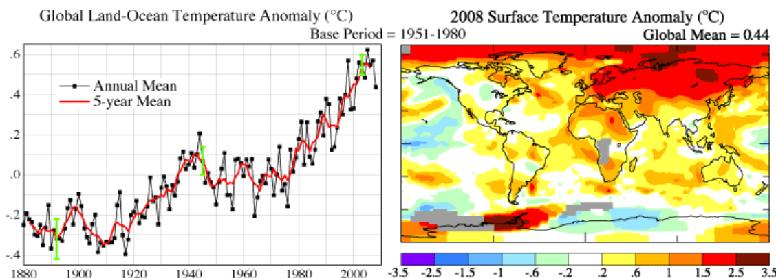
Figure A – Left: Annual-means of global-mean temperature anomaly Right: Global map of surface temperature anomalies, in degrees Celsius, for 2008. 8
