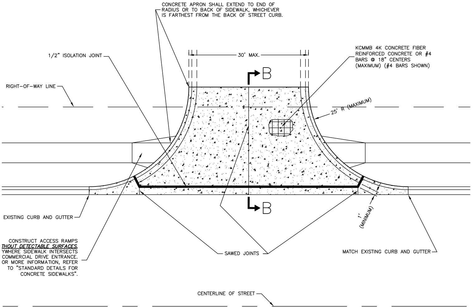
PLAN
