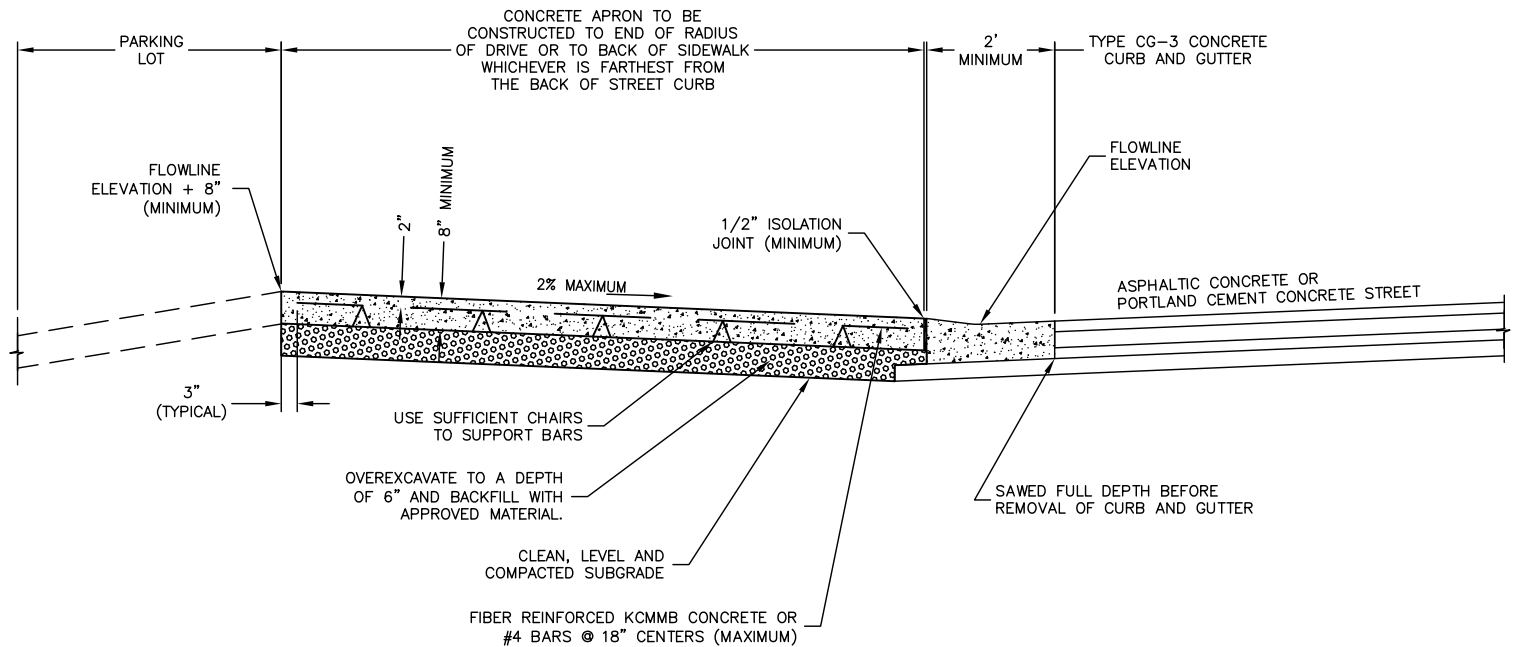
SECTION B-B
