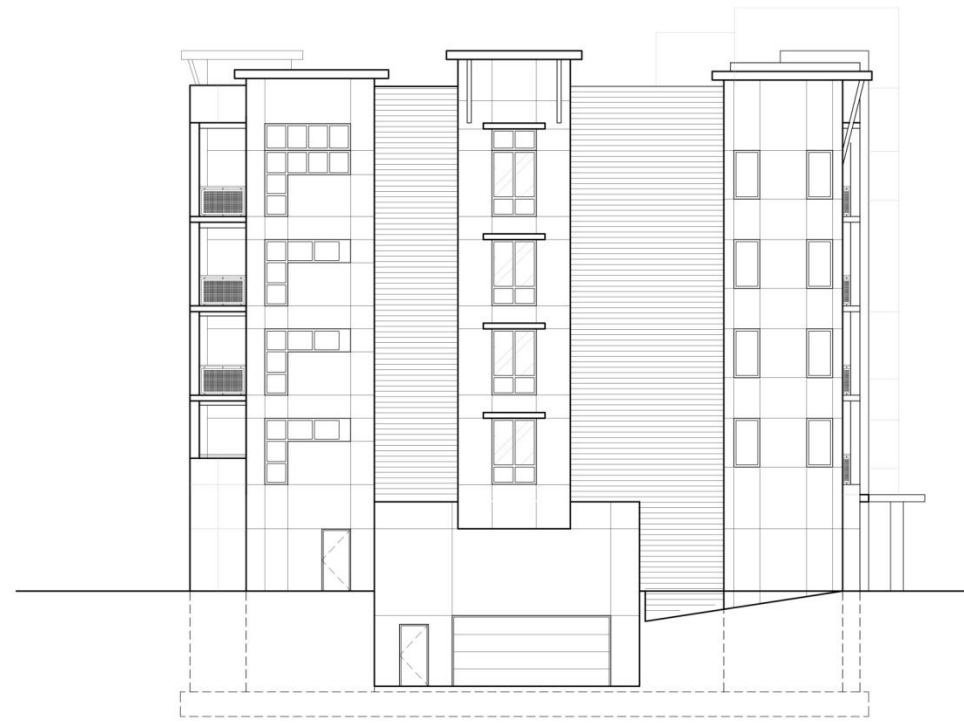
north elevation
