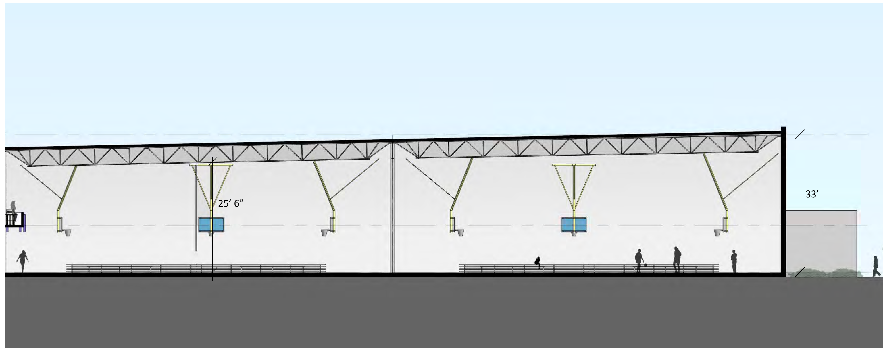
SECTION THROUGH FIELDHOUSE
