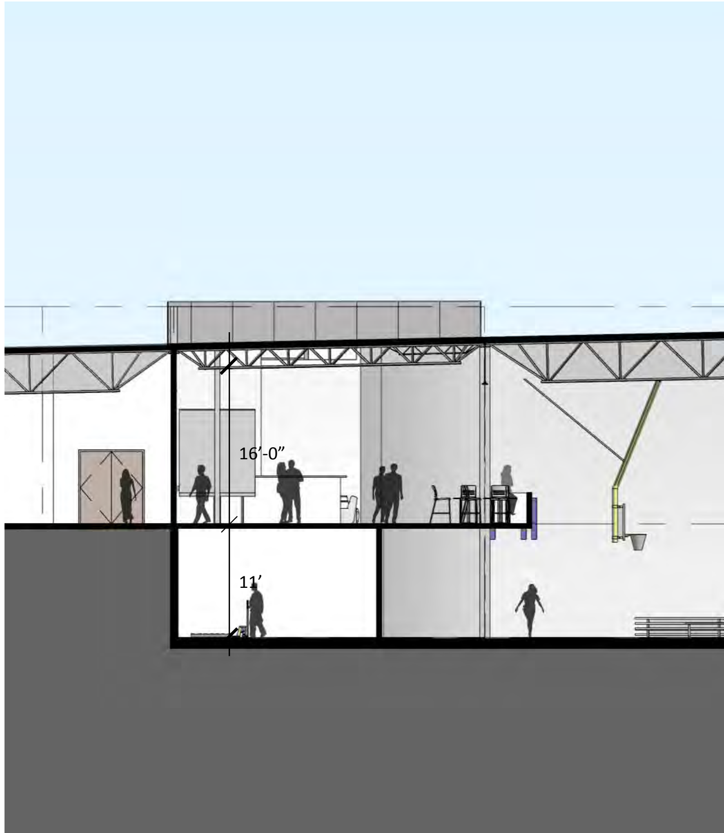
SECTION THROUGH MEZZANINE
