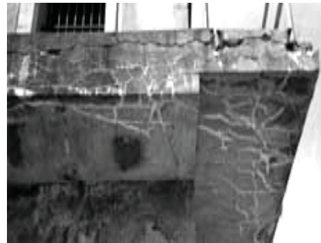
Common conditions of historic concrete – spalling (left) and cracking (right)
