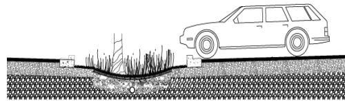
Site Section at parking with bio-swale
