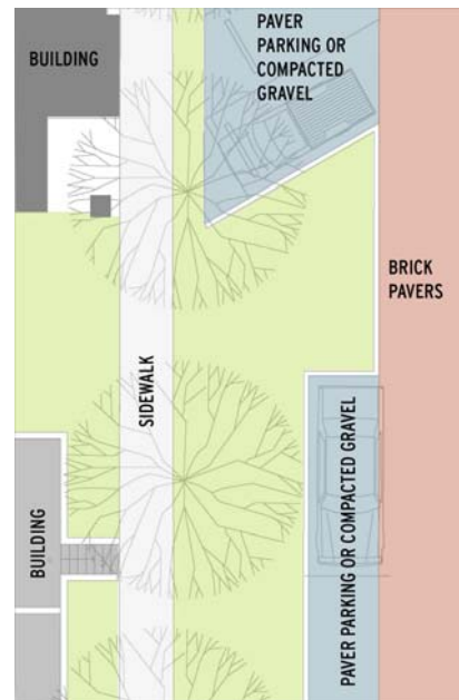
Pedestrian/Parking Surfaces - Mid Block Condition Shown here mid-block between 8 th and 9 th on the west side of Pennsylvania
