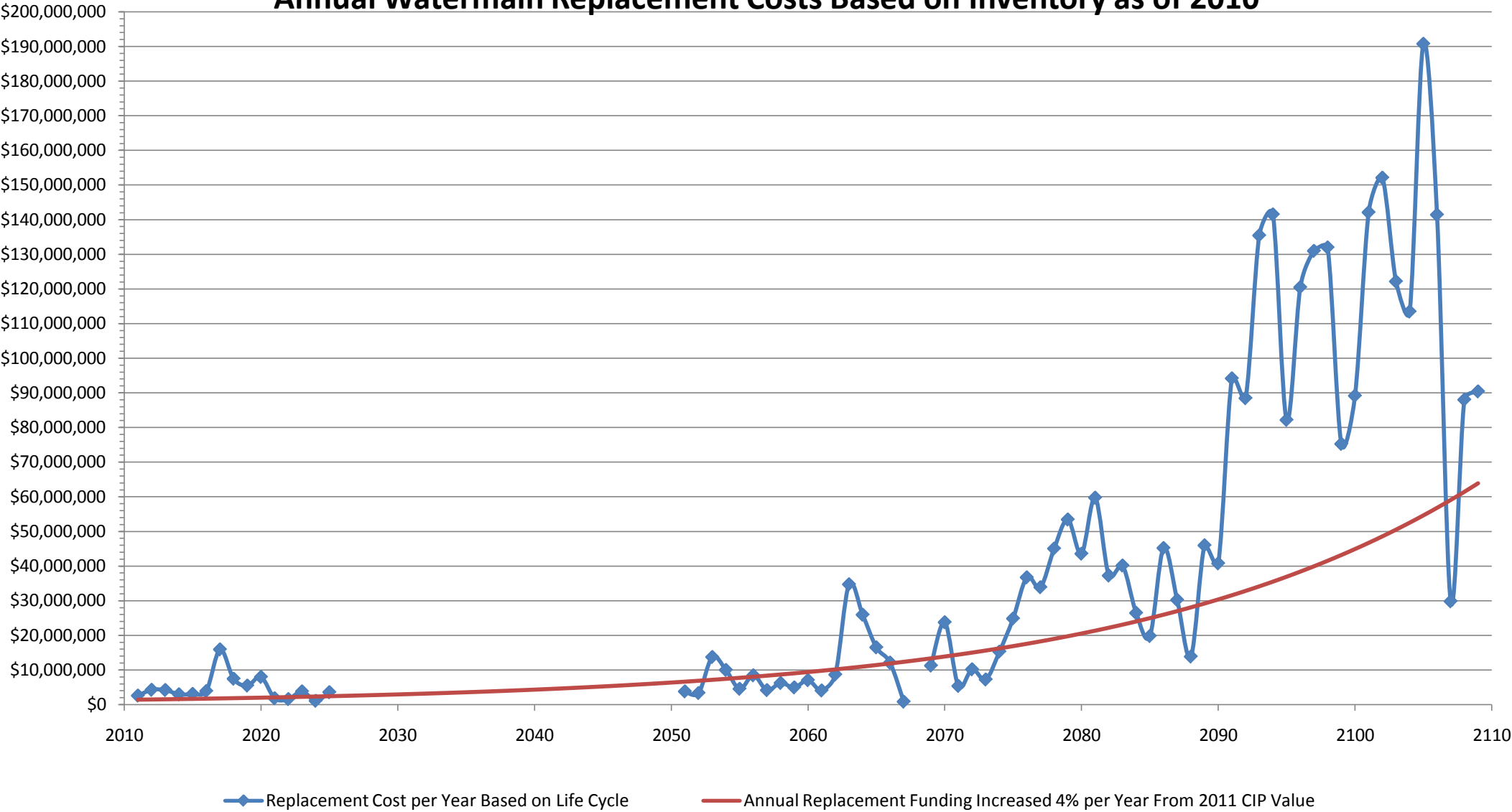
Annual Watermain Replacement Costs Based on Inventory as of 2010
