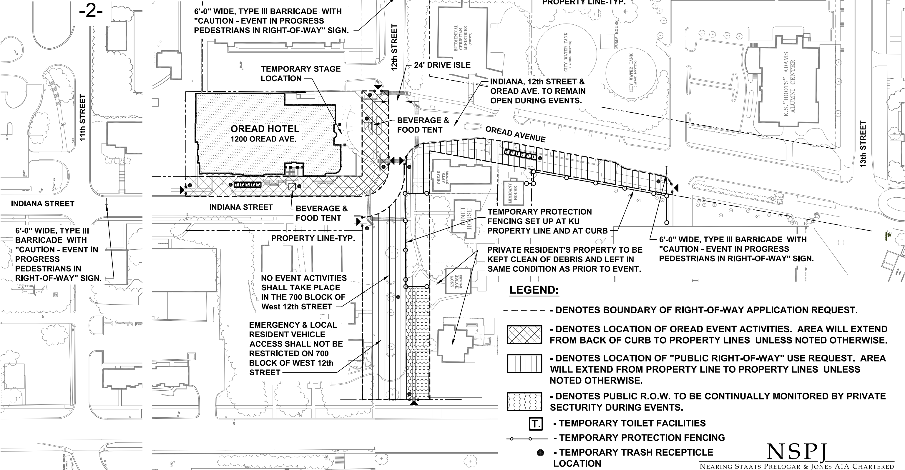
EXHIBIT PLAN "OREAD TAILGATE EVENT" NO SCALE
