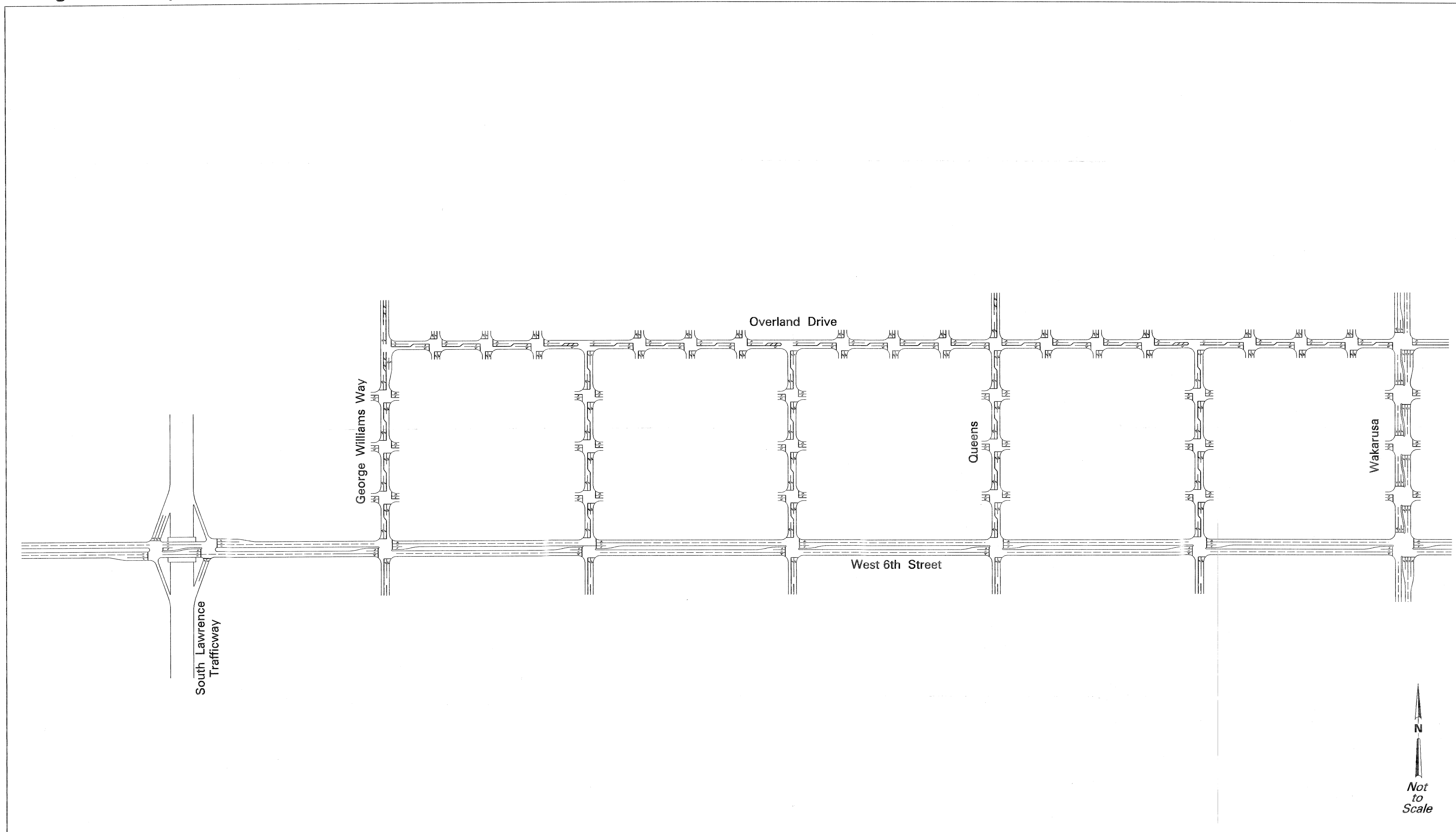
Figure 11 Scenario 3 (1/4 Mile Spacing) Lane Configuration
