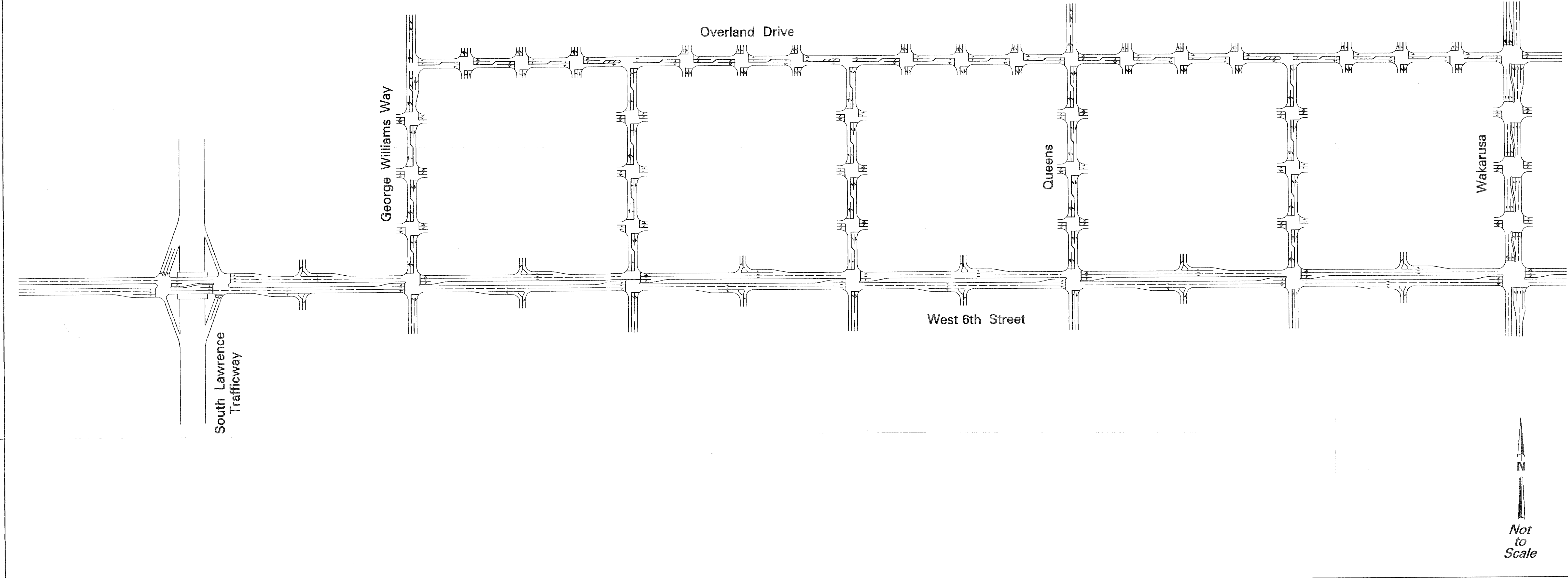
Figure 14 Scenario 4 (1/8 Mile Spacing) Lane Configuration
