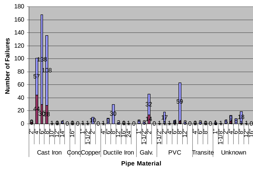
Waterline Failures - By Size & Material
