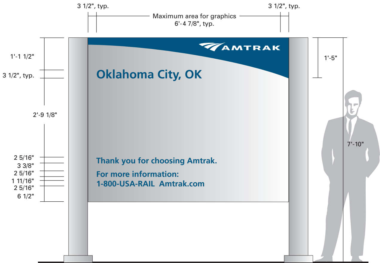
2 Kiosk Elevation - General Layout Side B SCALE: 1/2" = 1' - 0"
