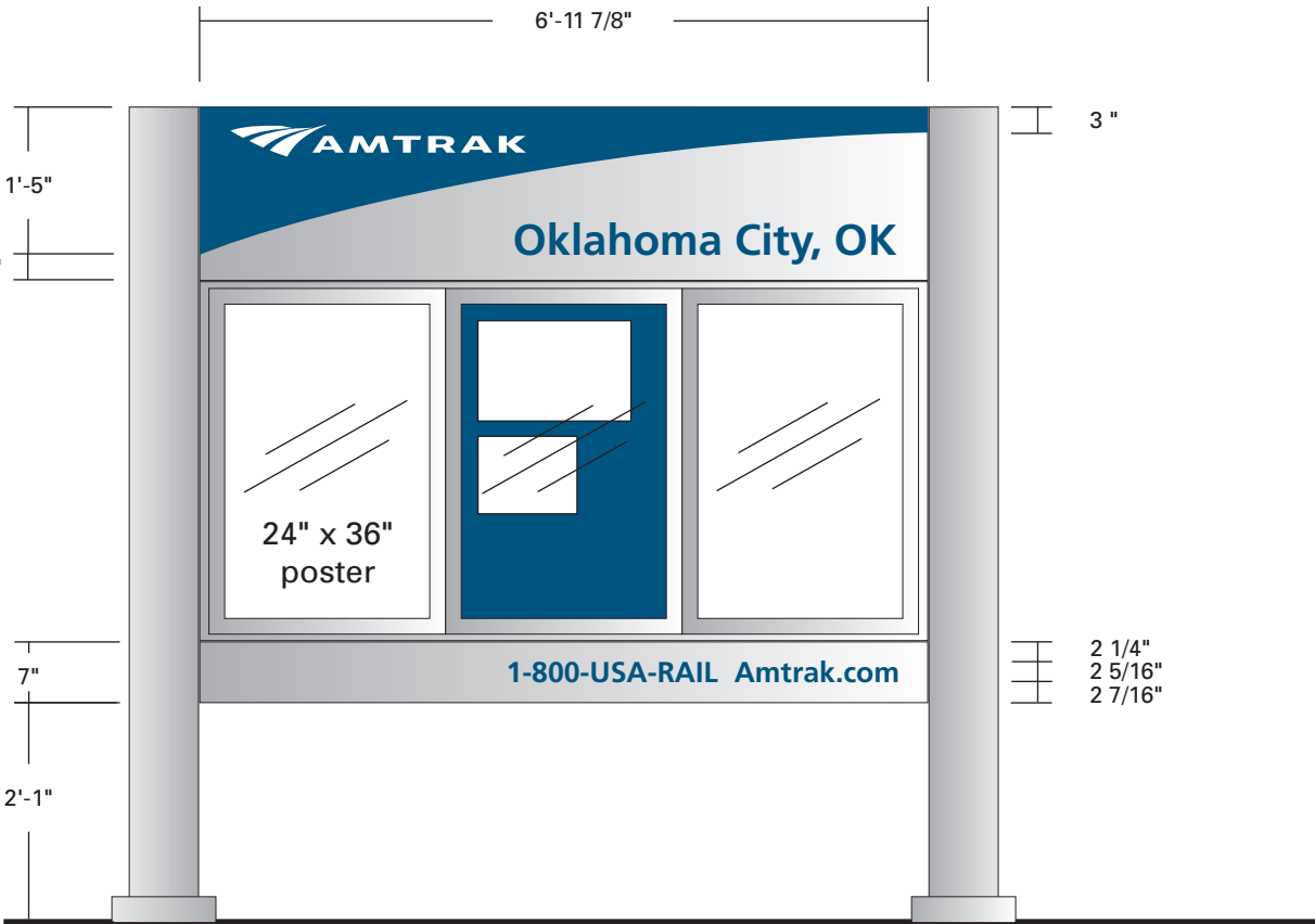
1 Kiosk Elevation - General Layout Side A SCALE: 1/2" = 1' - 0"
