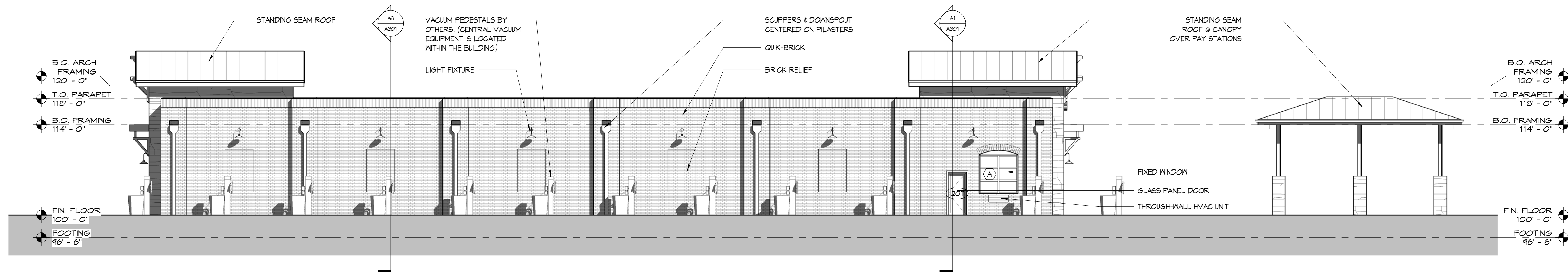
NORTH ELEVATION A1 1/8" = 1'-0"
