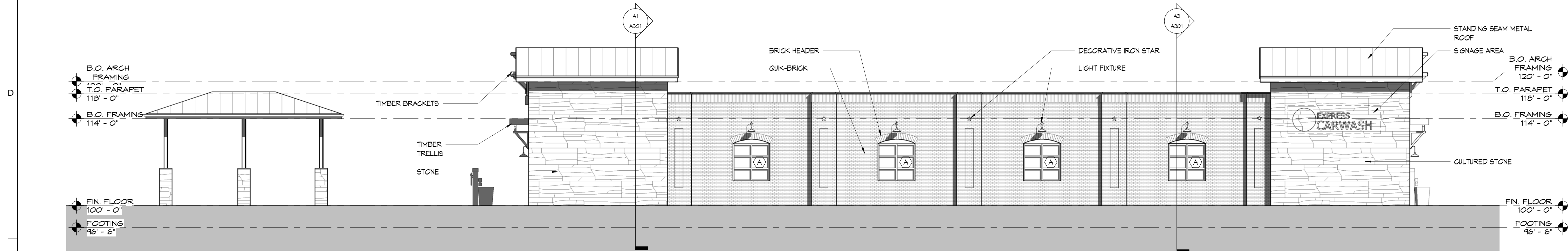
SOUTH ELEVATION C1 1/8" = 1'-0"
