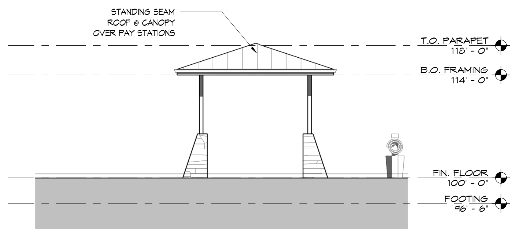
CARPORT WEST B5 1/8" = 1'-0"
