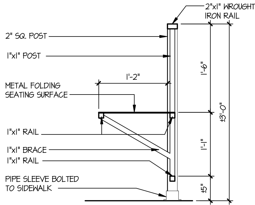
SECTION THROUGH RAILING SCALE: 1" = 1'-0"
