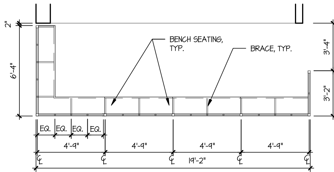
ENLARGED PLAN OF HOSPITALITY AREA SCALE: 1/4" = 1'-0"
