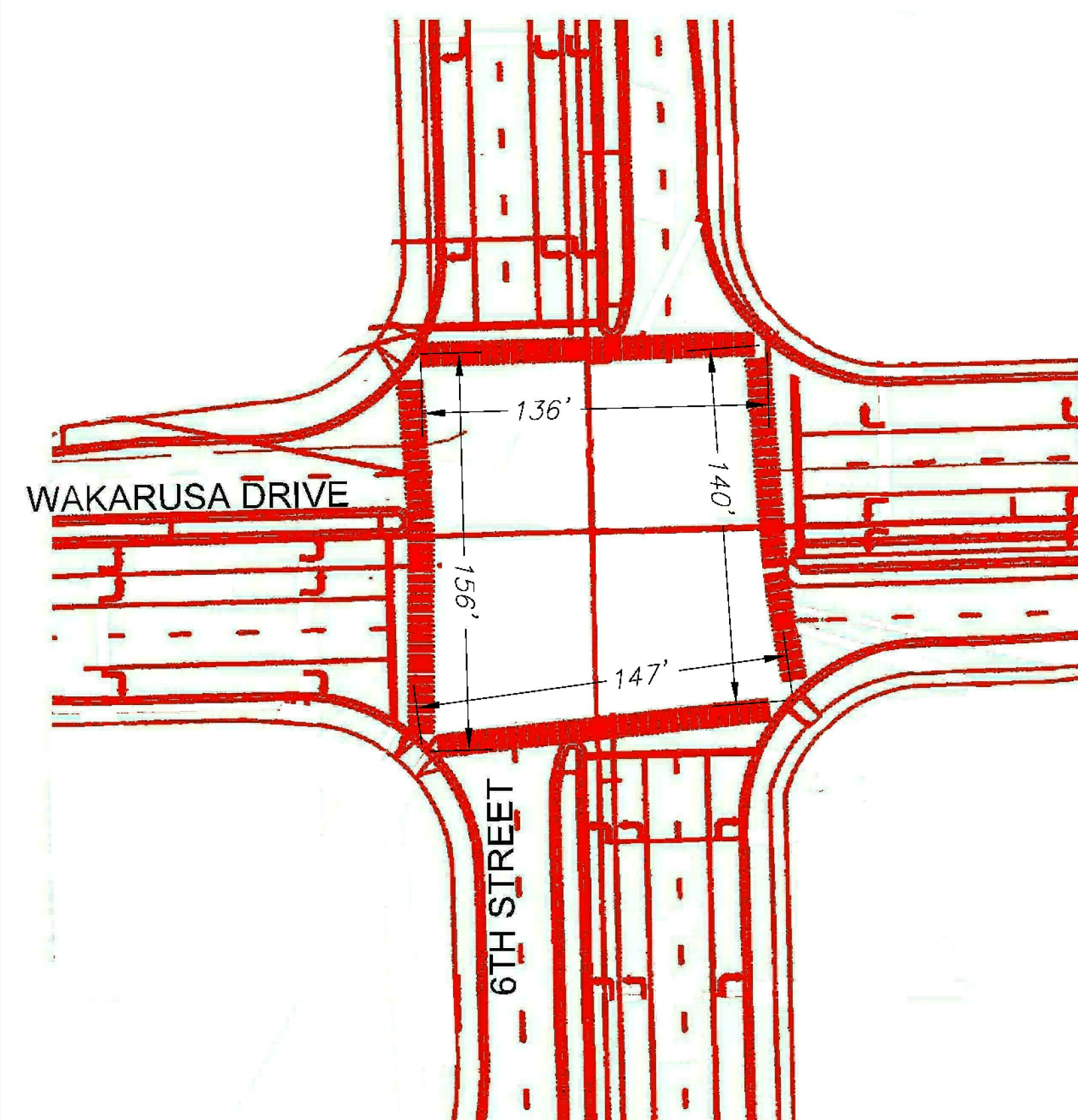
SIXTH AND WAKARUSA INTERSECTION
