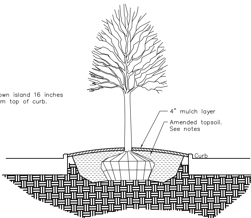
4 TYPICAL ISLAND - Section SCALE: NTS
