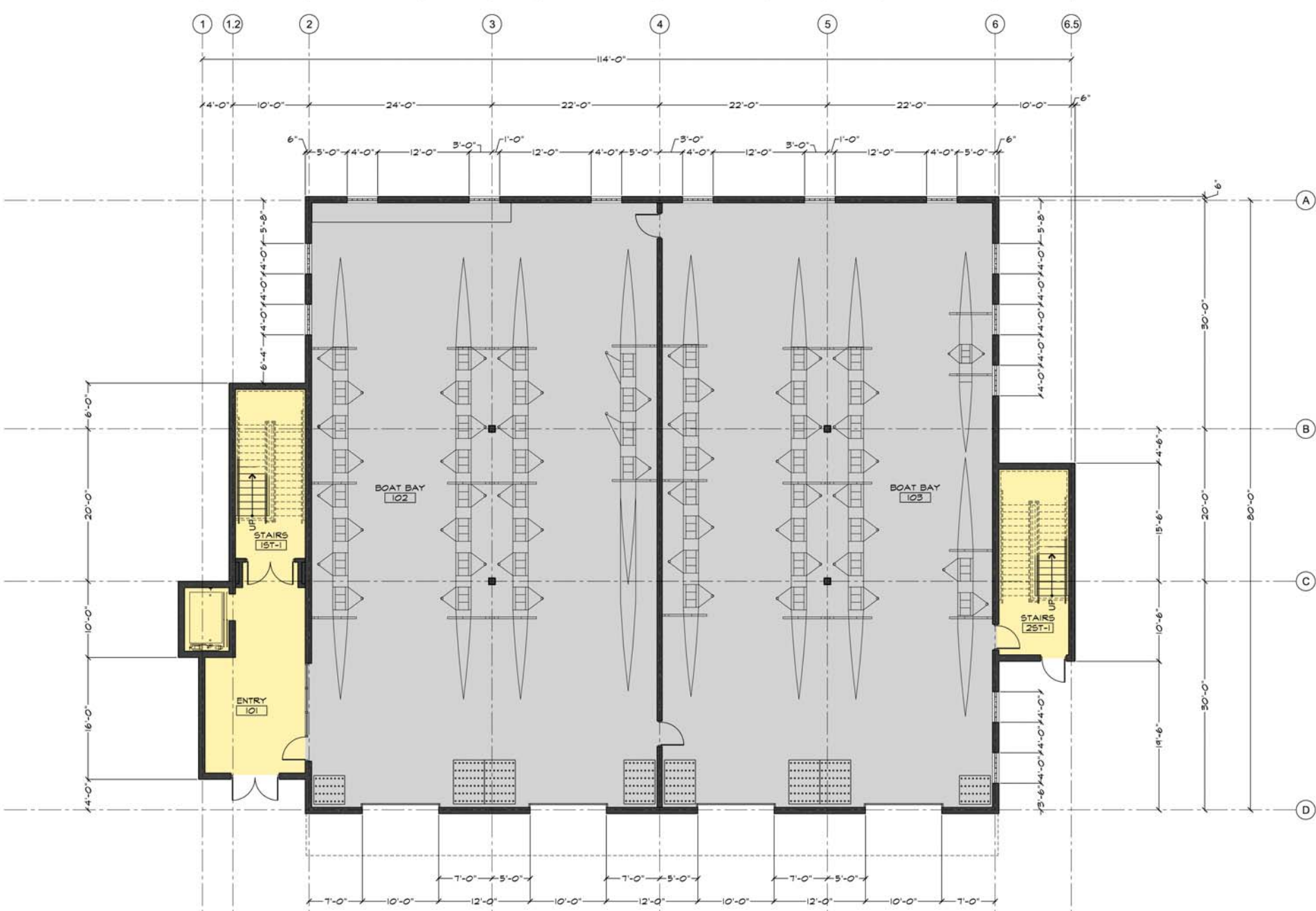
DRAWING: GROUND FLOOR PLAN
