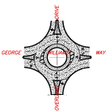
DOUBLE LANE ROUNDABOUT
