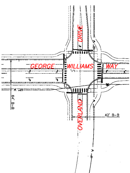
SIGNALIZED INTERSECTION
