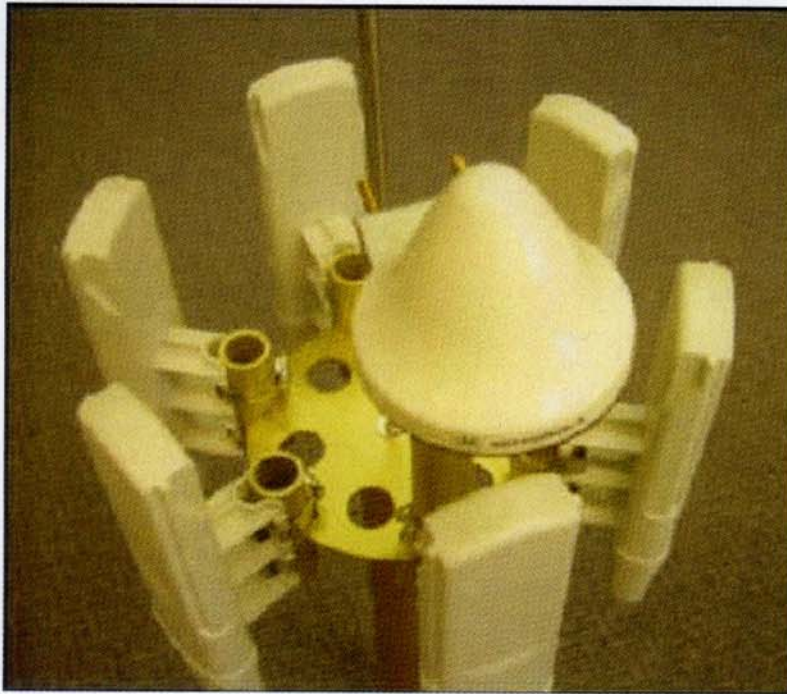
Figure 6 Motorola Canopy Cluster Mount
