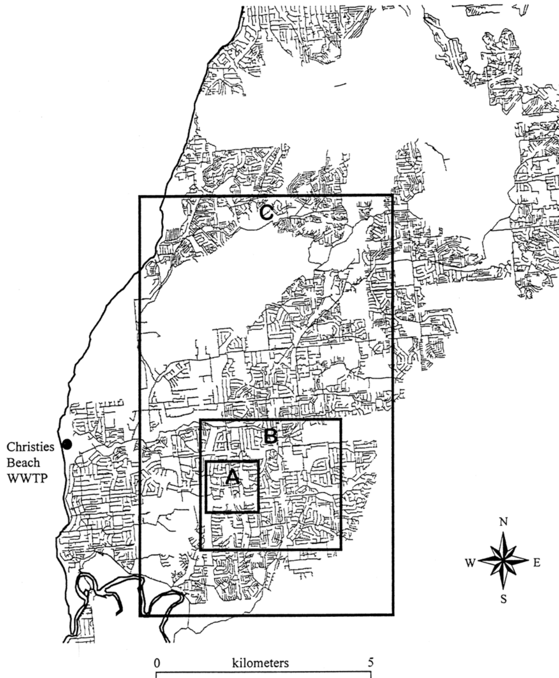
Figure 11-4: Example of Inclusion of Low-Density Areas as Scale of Service Expands. The lines shown represent the sewer network. Low-density (open space) areas are shown by the lack of lines. Source: Clark (1997), Figure 2.2. Courtesy of Richard Clark.
