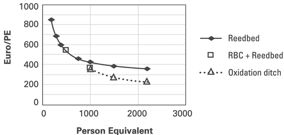
Figure 11-2: Capital Cost Per Person Equivalent for Wastewater Systems Serving 200 to 2,000 Person Equivalents in Belgium. Note: The reedbed technology is a two-stage reedbed; the RBC plus reedbed is a rotating biological contactor plus a simpler reedbed. Source: Adapted from Geenens and Thoeve (2000), Figure 5. Used by permission of the copyright holder, the International Water Association.
