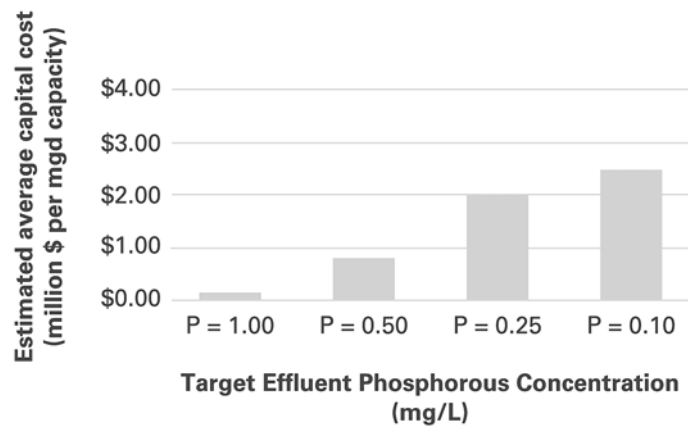
Figure 11-3: Estimated Unit Capital Costs to Achieve Specific Phosphorus Concentrations for 5 Small New England Wastewater Treatment Plants (January 1999 dollars, based on ENR20 cities index = 5,950). Source: Adapted from Freedman and Stallings (2000), Figure 2. Used by permission of the New England Water Environment Association.
