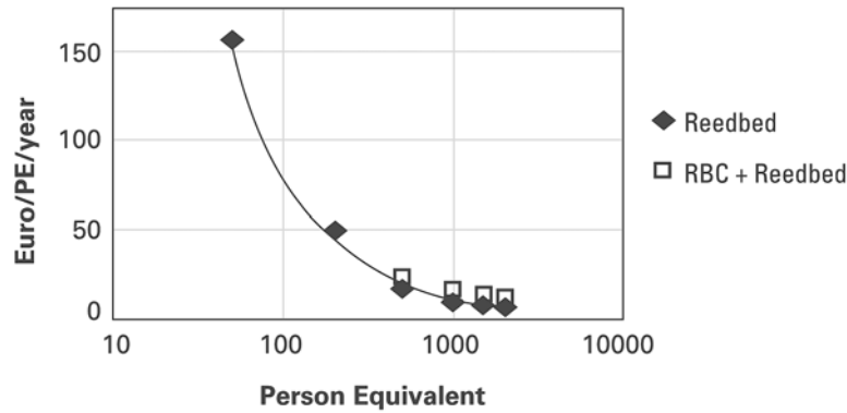
Figure 11-6: O&M Cost Per Person Equivalent for Small Wastewater Treatment Plants in Belgium.
