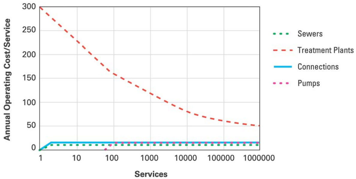
Figure 11-9: Service Scale Versus Operating Costs for Wastewater Systems in Adelaide, Australia. Costs are in 1997 Australian dollars. Source: Adapted from Clark (1997), Figure 4.2. Courtesy of Richard Clark.
