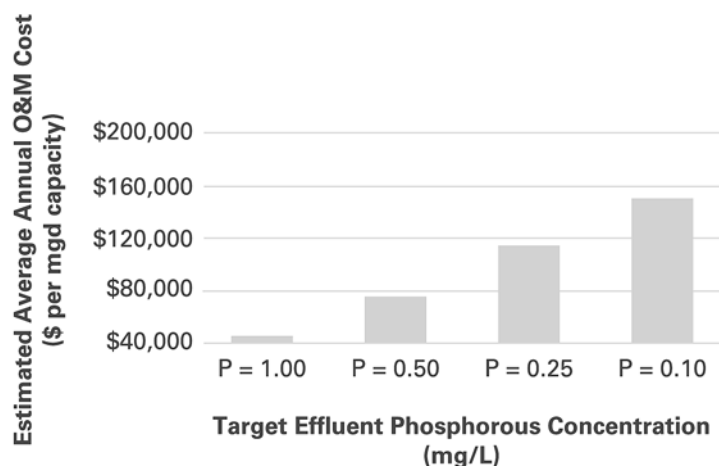
Figure 11-7: Estimated Unit O&M Costs to Achieve Specific Phosphorus Concentrations for 5 Small New England Wastewater Treatment Plants (January 1999 dollars, based on ENR20 cities index = 5,950). Source: Adapted from Freedman and Stallings (2000), Figure 3. Used by permission of the New England Water Environment Association.
