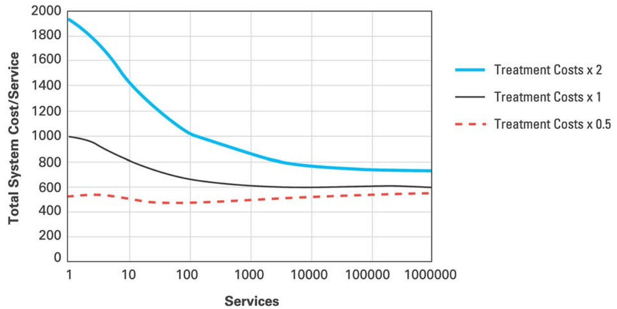
Figure 11-11: Total Annual Costs Per Service, at Varying Treatment Plant Capital Costs, for Wastewater Systems in Adelaide, Australia. Costs are in 1997 Australian dollars. Source: Adapted from Clark (1997), Figure 4.3b. Courtesy of Richard Clark.
