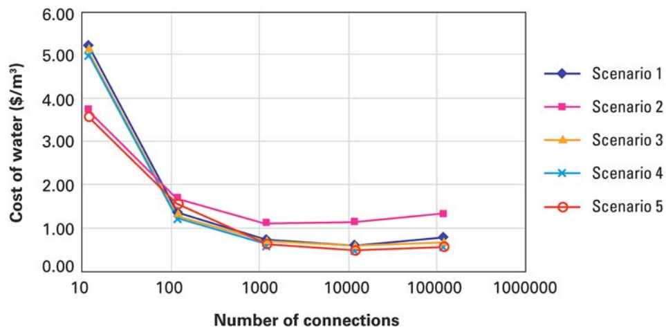
Figure 12-1: Total Cost of Water by Scale of Service for 5 Hypothetical Graywater Reuse Options. Source: Adapted from Booker (1999), Figure 11. Courtesy of the Commonwealth Scientific and Industrial Research Organization (CSIRO).
