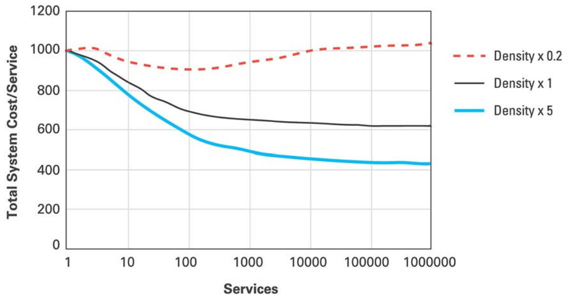
Figure 11-10: Total Annual Costs Per Service, at Varying Population Density, for Wastewater Systems in Adelaide, Australia. Costs are in 1997 Australian dollars. Source: Adapted from Clark (1997), Figure 4.3a. Courtesy of Richard Clark.
