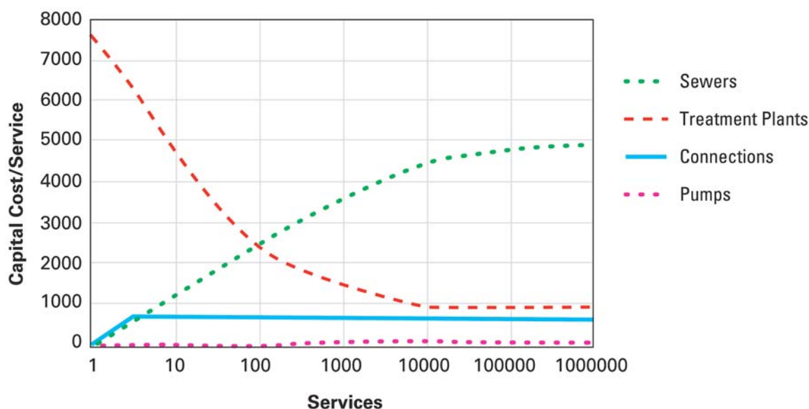
Figure 11-8: Service Scale Versus Capital Costs for Wastewater Systems in Adelaide, Australia. Costs are in 1997 Australian dollars. Source: Adapted from Clark (1997), Figure 4.1. Courtesy of Richard Clark.
