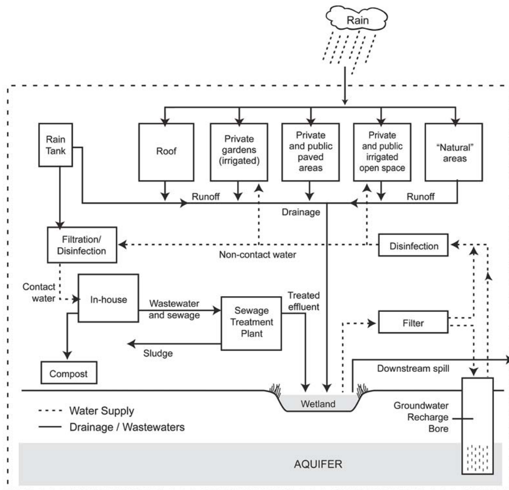
Figure 12-2: Integrated Water, Wastewater, and Drainage Scheme. Source: Adapted from Clark (1997), Figure 5.2. Courtesy of Richard Clark.
