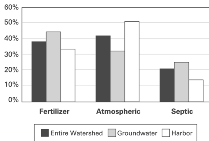
Figure 9-1: Proportion of Nitrogen from 3 Sources Over 5 Years to the Watershed, Ground Water, and Harbor of Solomon's Harbor, Maryland. Source: Adapted from Voinov et al. (2004), Figure 4. Courtesy of Alexey Voinov.
